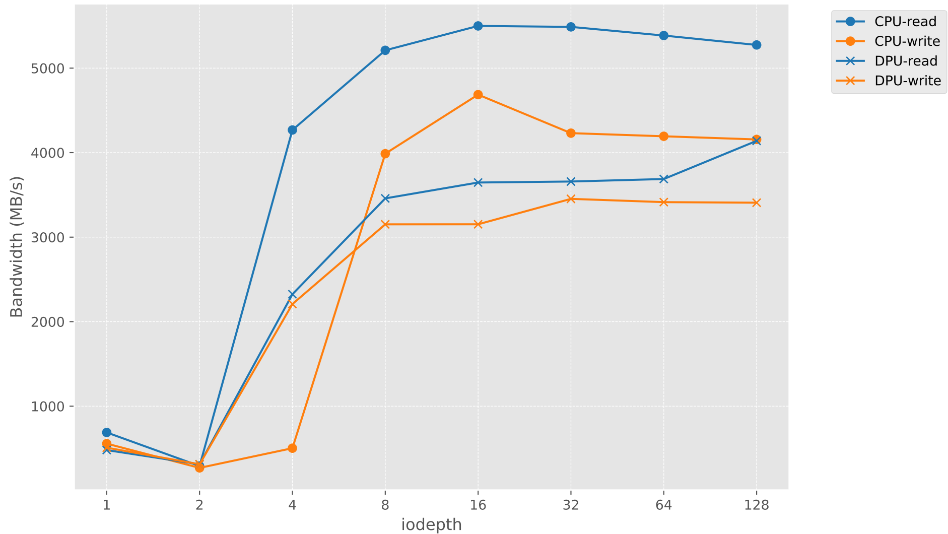
Bandwidth vs iodepth (Sequential)
